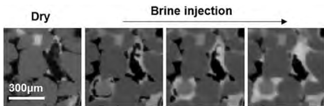
Figure 5. Example of two-dimensional views of oil phase trapping in pores under water-wet condition.
