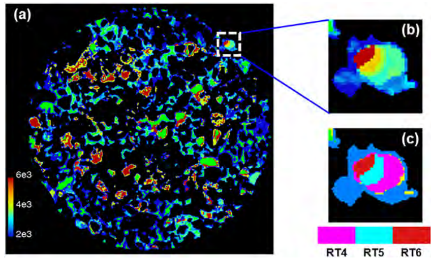
Figure 10. (a) A slice of invasion capillary pressure distribution on X - Y plane of the mixed-wet sample. The “capillary instability pores” are marked in green. (b) A zoom in view of “pressure distribution” in pore (a). Note that the pressure in “gradually filling pores” does not have the same meaning as in the microporosity. It only represents the moving sequence of fluid-fluid interfaces in macropores, that is, “low pressure region” is invaded first, followed by the “high pressure region.” (c) An example of “rock typing” results for pore A in model (b). The segmentation of RT1-RT3 in model B is the same as model A, see Figure 9b. The RT4, RT5, and RT6 represent gradually filling zones.
