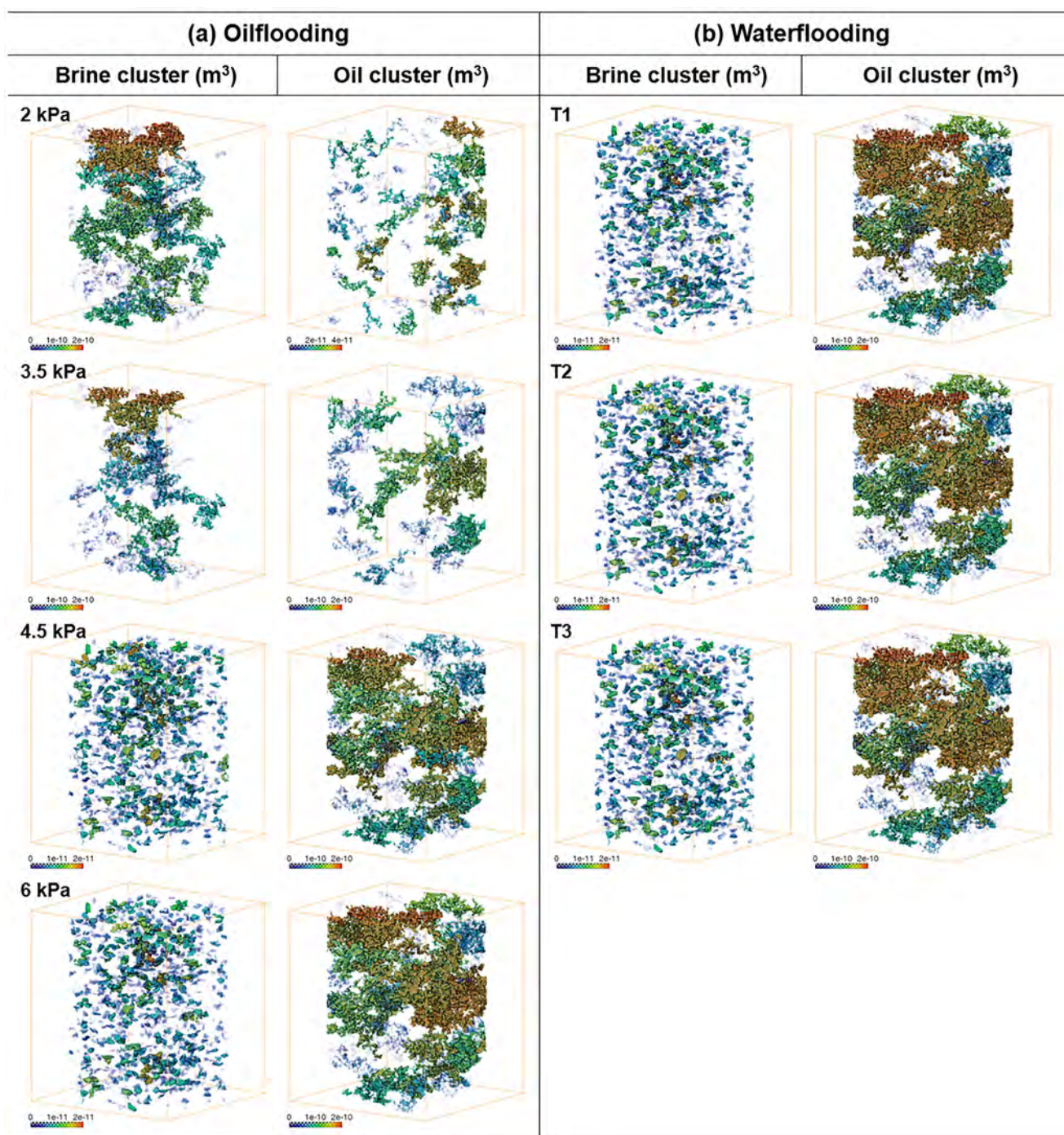
Figure 6. Fluid cluster changes in macropores of the mixed-wet sample during (a) oilflooding and (b) waterflooding. The color shows cluster volume ( \text{m}^3 ).
