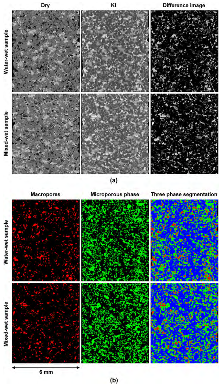
Figure 2. (a) Two-dimensional cross-sections of filtered water-wet and mixed-wet samples. The left, middle, and right columns show dry scan, brine-saturated scan, and the difference image between brine-saturated scan and dry scan. (b) The segmented macropores (left), microporous phase (middle), and all phases (right) for both samples. The red, green, and blue phases represent macropores, micropores, and solid grain.
