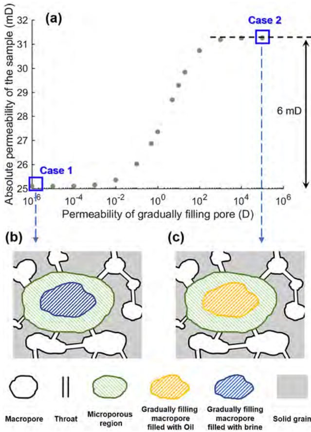
Figure 11. (a) Simulation results of the input permeability value for gradually filling pores and the absolute permeability of the sample. (b) Diagram of the gradually filling pore blocked by brine at very low permeability condition during two phase flow. (c) Diagram of the gradually filling pore blocked by oil at very high permeability condition during two phase flow.
